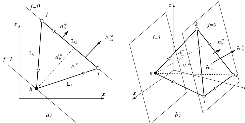
Figure 16 : Since the shape function is equal to one in one vertex and zero in the other vertices, the modulus of its gradient is the inverse of the distance between the corresponding vertex and it opposite side (or its opposite face in 3D).
