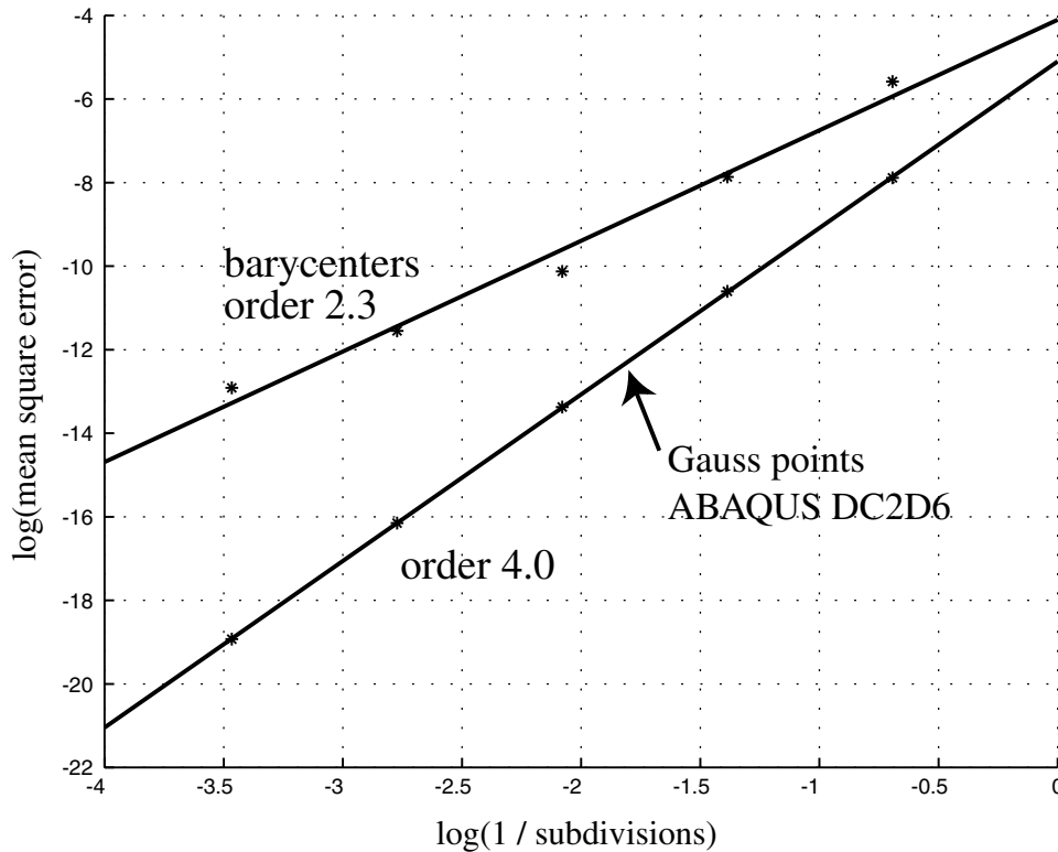
Figure 14 : The order of convergence of the two subdivisions.
