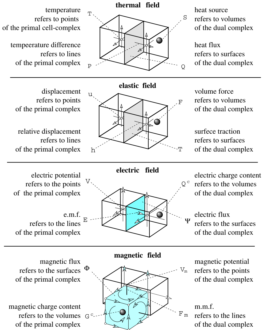
Figure 4 : Physical variables and cell complexes
