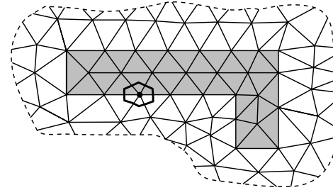
Figure 7 : Thermal generation uniformly distributed in a subregion.
