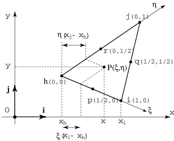
Figure 9 : Relation between the global cartesian coordinates and local affine coordinates.
