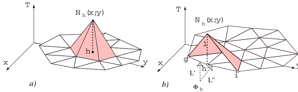
Figure 15 : The nodal shape functions: a) for an internal node; b) for a boundary node.
