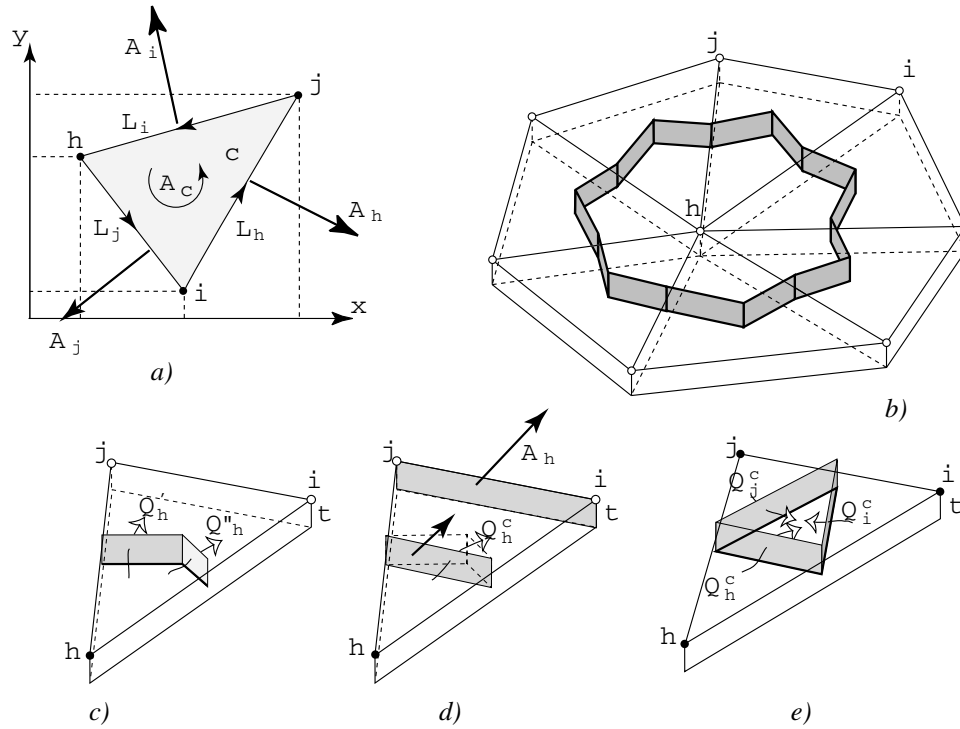
Figure 6 : a) The elements of triangle. b) The dual polygon conceived as a prism. c) the heat flux relative to the node h and d) its equivalent; e) the three heat fluxes associated with the three vertices.
