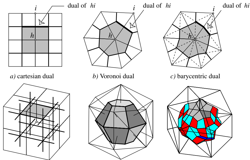
Figure 3 : Primal and dual cell complexes.
