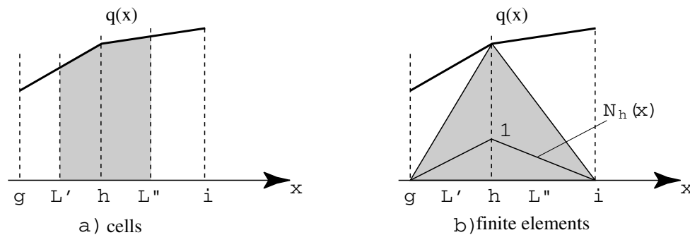
Figure 17 : The boundary heat fluxes evaluated: a) by cell method; b) by FEM.
