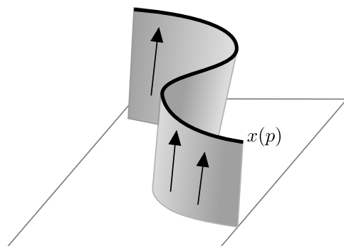
Figure 1: The one-dimensional set x(p) (in black) intersects transversely all the orbits lying in a portion of the stable manifold (in grey).
