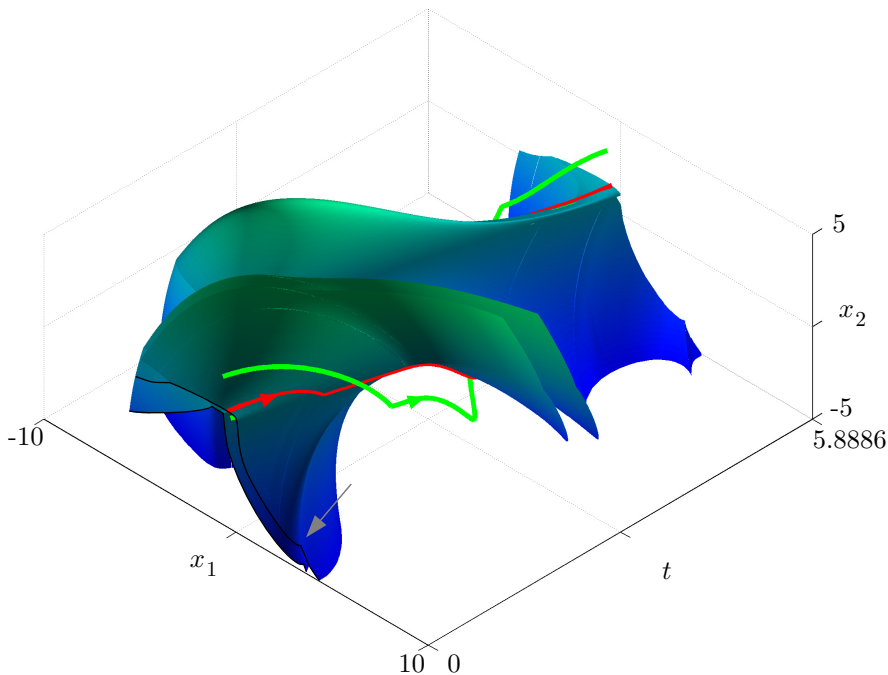
Figure 9: The blue surface is the stable manifold of the saddle cycle. Orbits of the manifold were continued backward in time up to their first intersection with the surfaces x_2 = \pm 5 . The red and green cycles are respectively the saddle cycle and the two stable ones. The intersection of the stable manifold with the plane t = 0 , plotted here in black, correspond to the boundary represented in Fig. 8. Part of the boundary appearing in Fig. 8 is not shown in this figure, since it is generated by orbits that extend beyond the interval x_2 \in [-5, +5] . The arrow in the lower left part of the figure indicates the crease mentioned in Fig.8.
