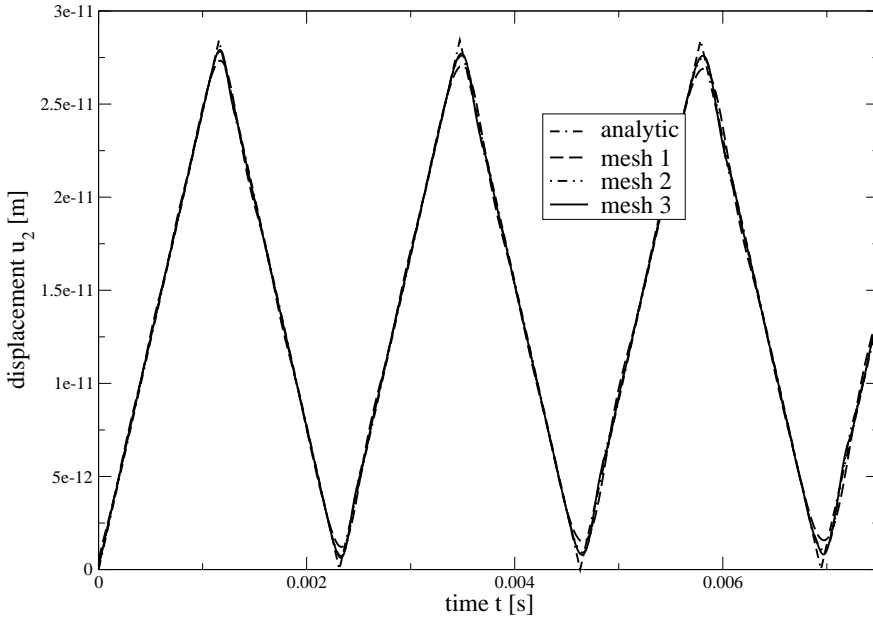
(a) Displacement at the top
