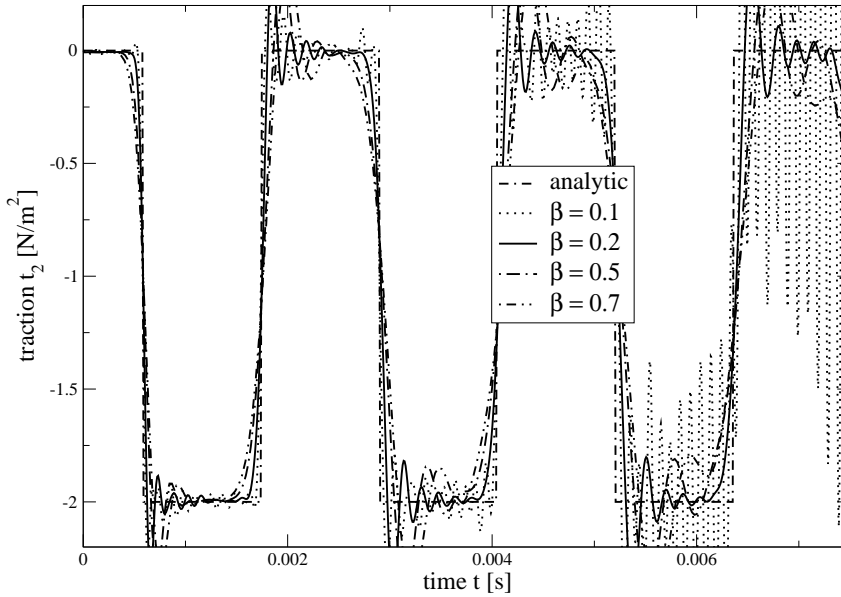
(b) Traction at the bottom
