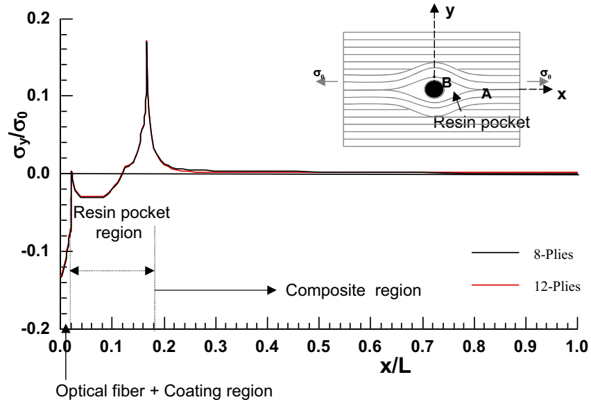
Figure 14 : Variation of \sigma_y along x-axis over the complete length
