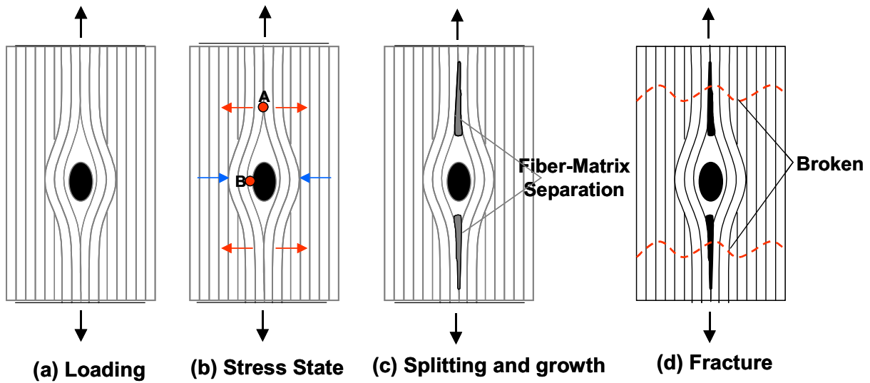
Figure 4 : Tensile Failure Process for Composite Laminate Embedded with Optical Fiber at 90 ° to the Load Axis [Emmanwori (2002), Shivakumar and Emmanwori (2002)]
