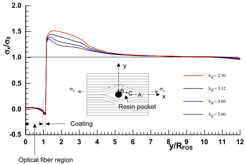
Figure 18 : Variation of Normalized \sigma_x along y-axis for various h_d/R_{FOS} values
