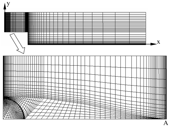
Figure 8 : Global and local finite mesh at critical locations
