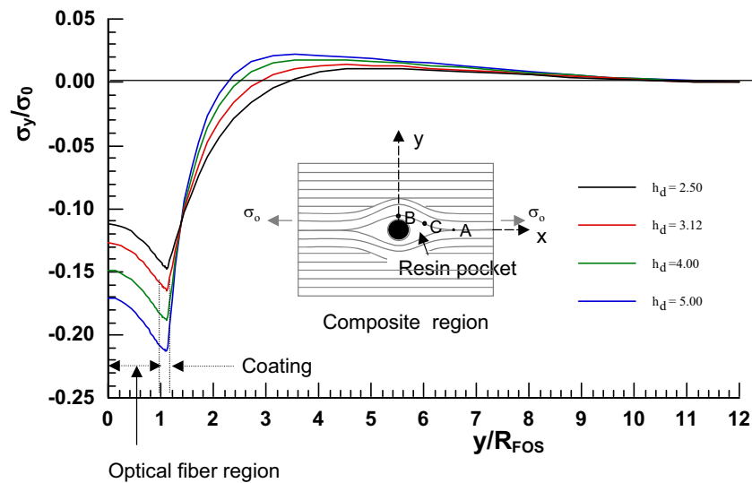
Figure 19 : Variation of Normalized \sigma_y along y-axis for various h_d/R_{FOS} values
