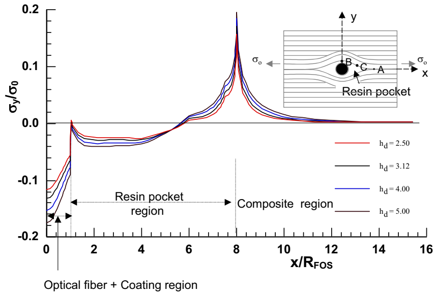
Figure 17 : Variation of Normalized \sigma_y along x-axis for various h_d/R_{FOS} values
