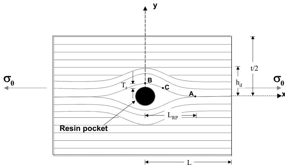
Figure 3 : Idealized model
