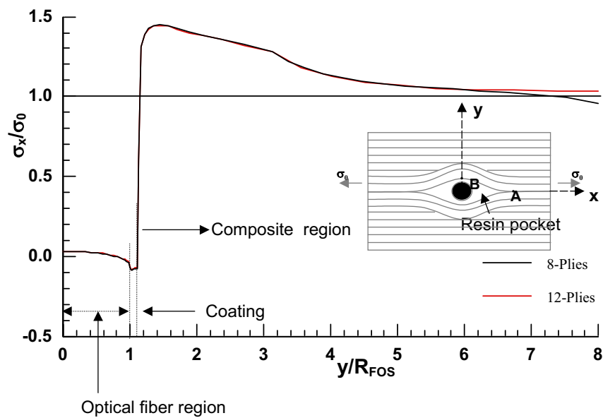
Figure 15 : Variation of \sigma_x along y-axis
