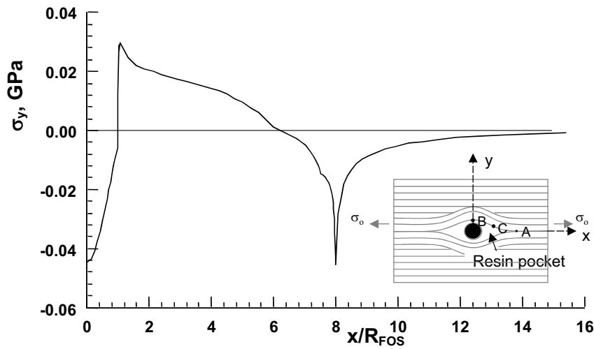
Figure 20 : Variation of \sigma_y along x-axis due to \Delta T = -175 °F
