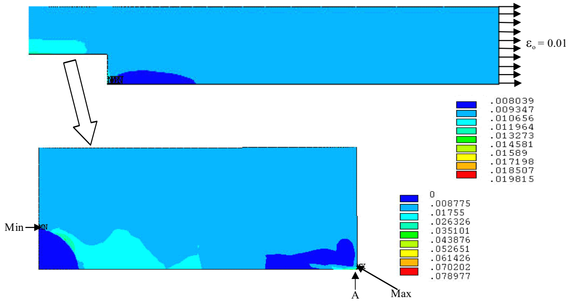
Figure 9 : Maximum principal ( \epsilon_1 ) strain contours (global and local views)
