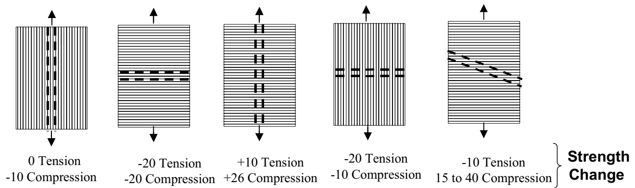
Figure 1 : Strength Reductions Due to FOS Orientation (Broken cylinders represent the fiber optic sensor)
