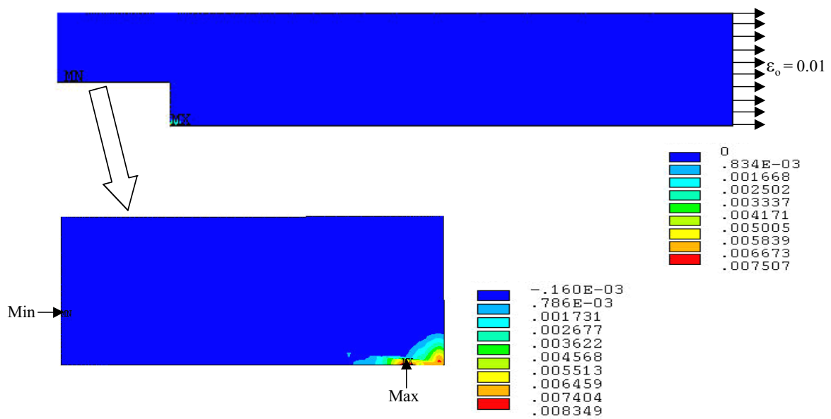
Figure 10 : Minimum principal ( \epsilon_2 ) strain contours (global and local views)
