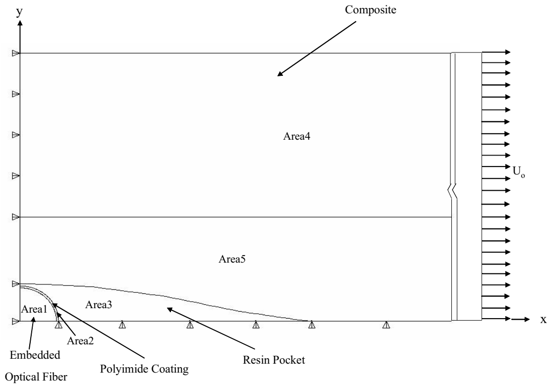
Figure 7 : Descritization of various regions
