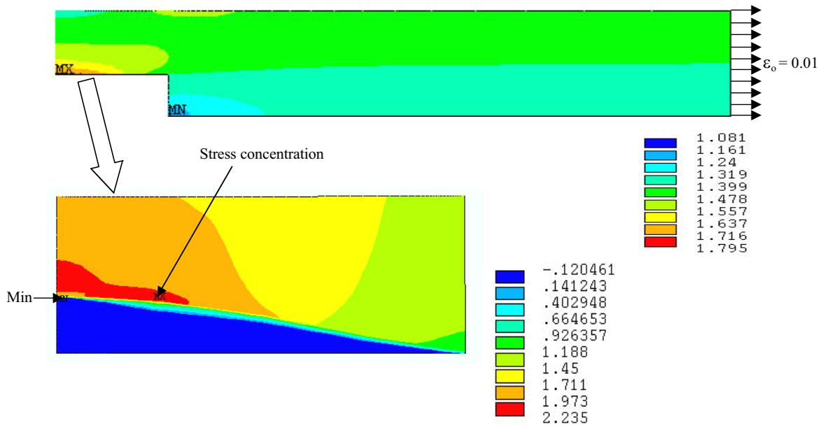
Figure 11 : Maximum principal ( \sigma_1 ) stress contours ( \sigma_o = 1.404 GPa, global and local views)
