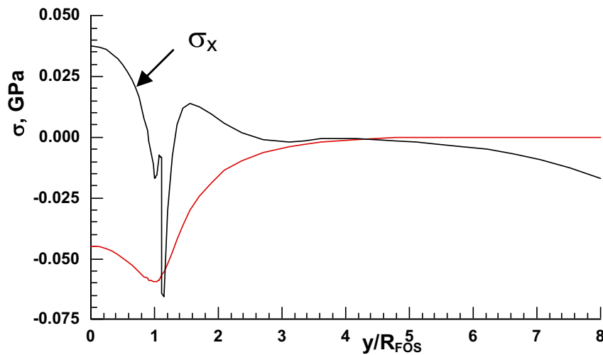
Figure 21 : Variations of \sigma_x and \sigma_y along y-axis due to \Delta T = -175 °F
