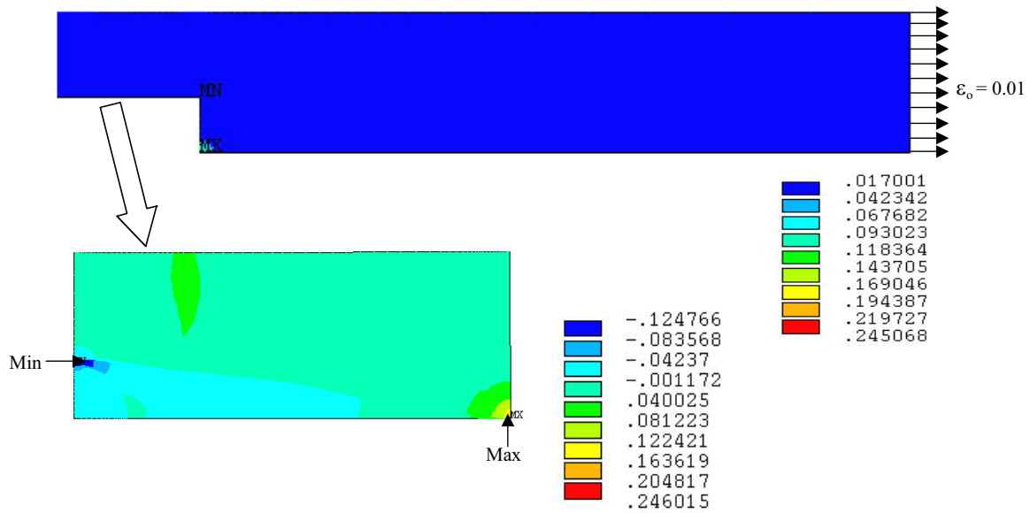
Figure 12 : Minimum principal ( \sigma_2 ) stress contours ( \sigma_o = 1.404 GPa, global and local views)
