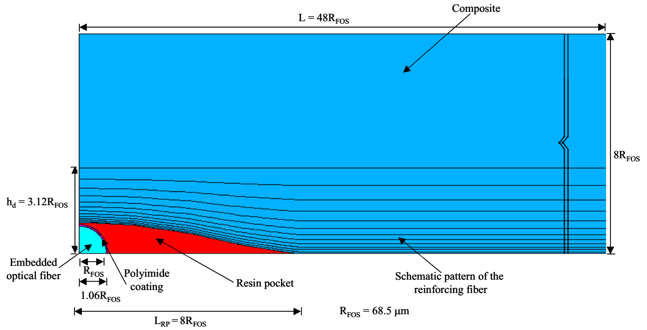
Figure 6 : One-quarter of the idealized model
