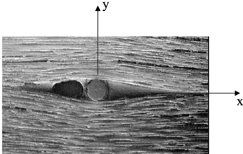
Figure 2 : Micrograph of section of composite laminate embedded with FOS
