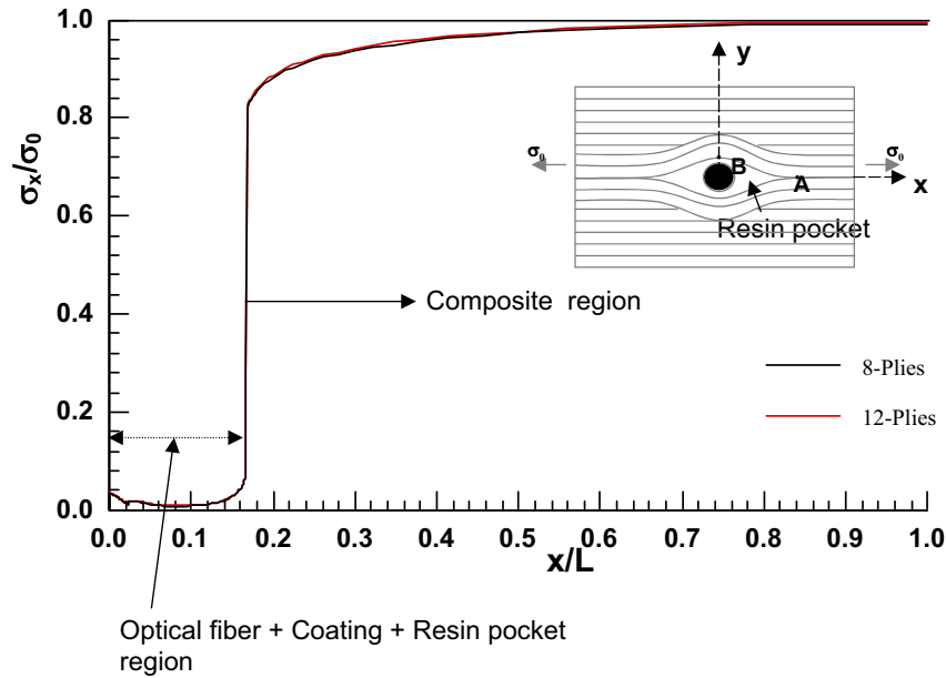
Figure 13 : Variation of \sigma_x along x-axis over the complete length
