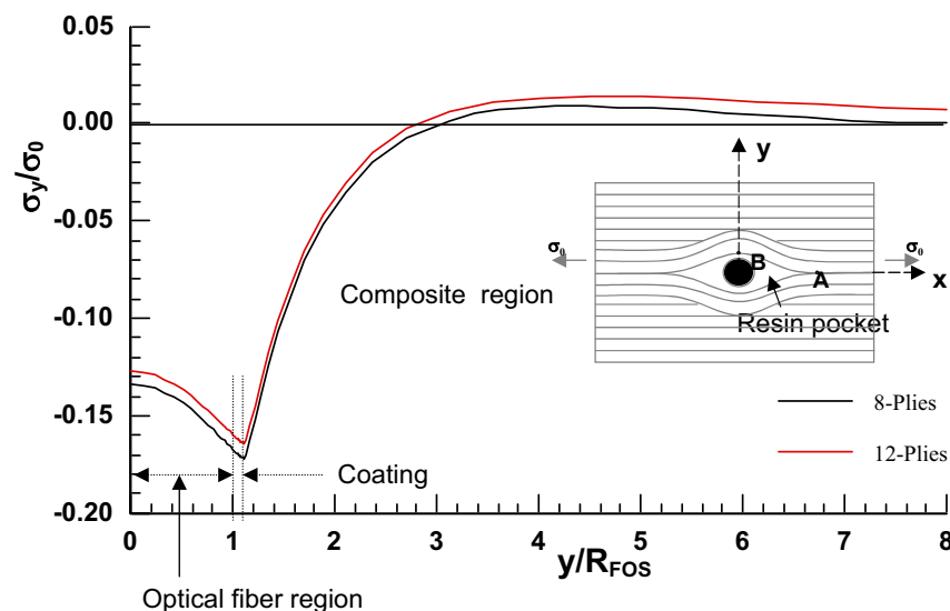
Figure 16 : Variation of \sigma_y along y-axis
