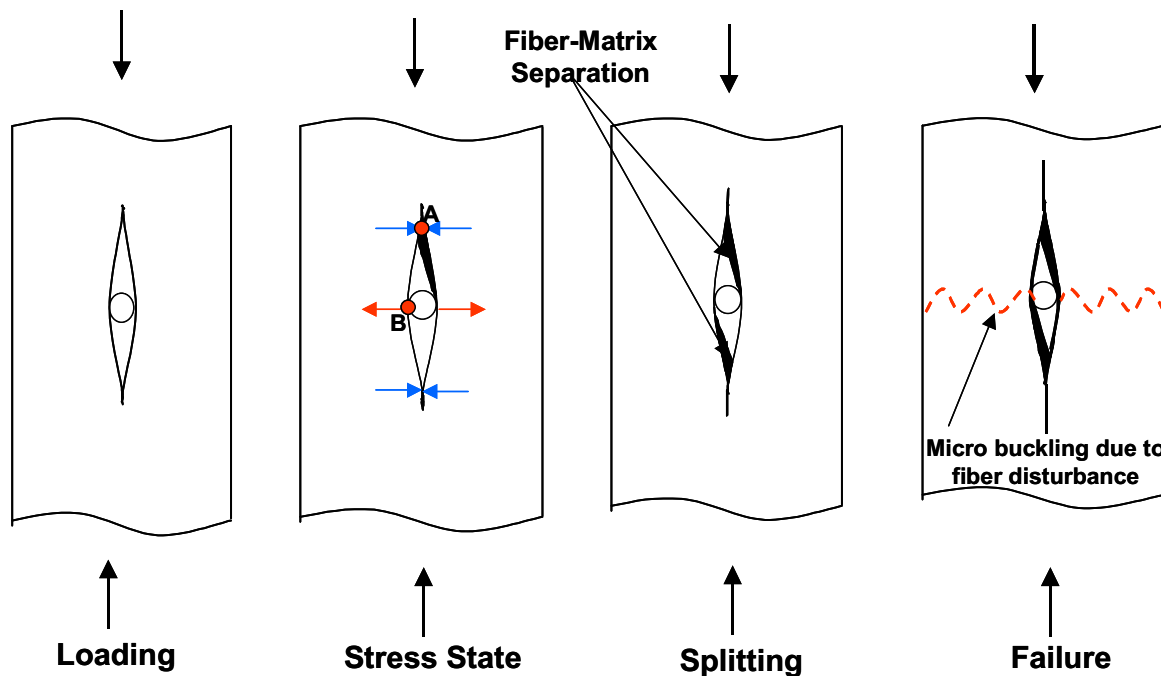
Figure 5 : Compression Failure Process for Composite Laminate Embedded with Optical Fiber at 90 ° to the Load Axis [Emmanwori (2002), Shivakumar and Emmanwori (2002)]
