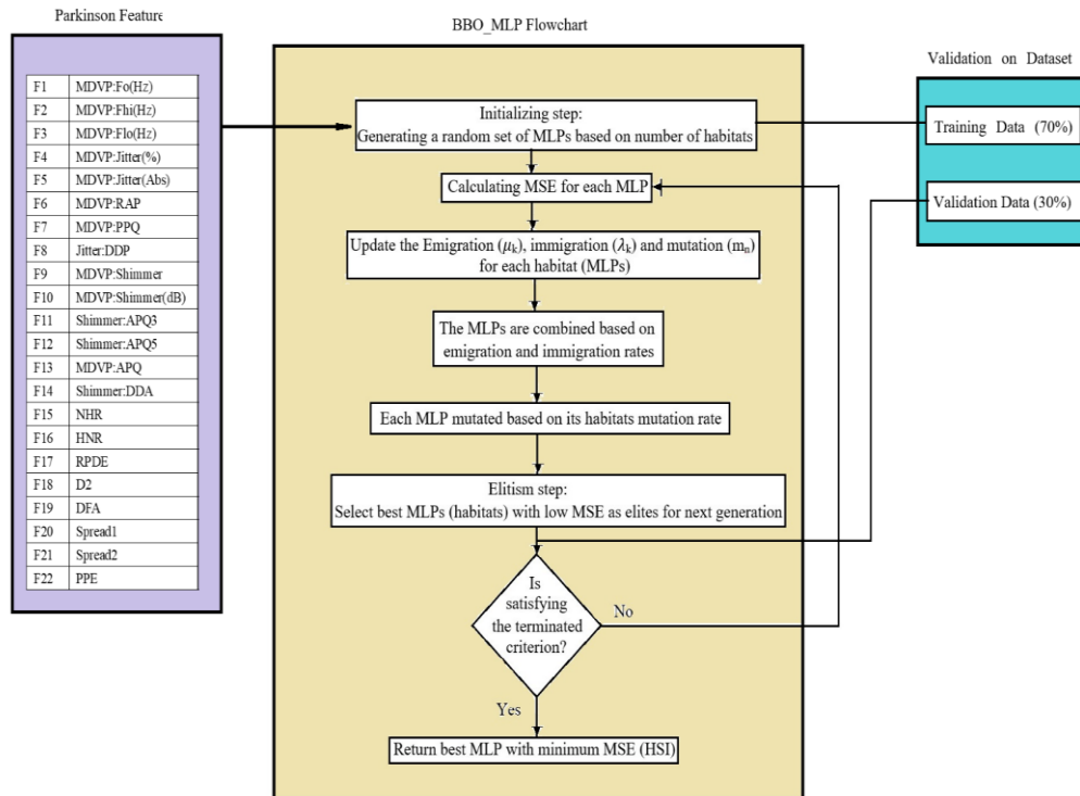
Figure 2: Flow chart of BBO_MLP Method
