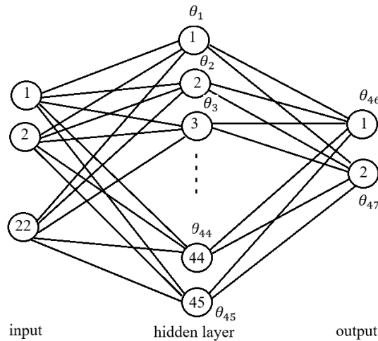
Figure 1: MLP with three layers [3]
