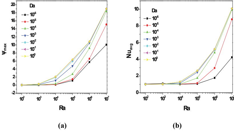
Figure 3: Influence of Ra and Da on Nu_{\text{avg}} and \psi_{\max} for XP = 0.2 , \varepsilon = 0.4 .
