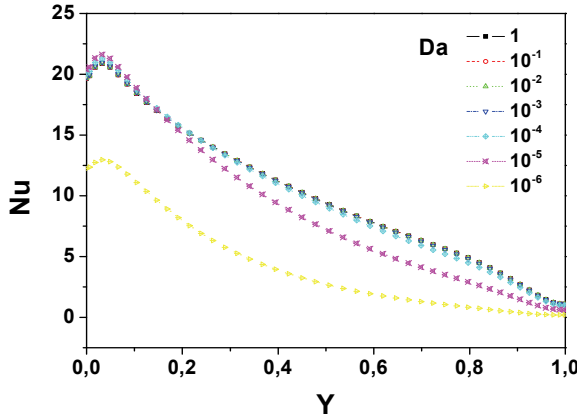
Figure 4: Local Nusselt number distribution on the right heated surface for different permeability of the porous layer Da and with, Ra = 10^7 , XP = 0.2 and \varepsilon = 0.4 .
