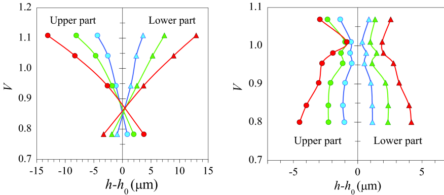
Figure 21: Extrema of the dynamic deformation at upper (circles) and lower (triangles) parts of a liquid bridge as a function of volume ratio V . The different curves with symbols (in order by the distance from the axis) correspond to the gas velocity U_0^g = 1 \text{ m/s} , 1.5 \text{ m/s} and 2 \text{ m/s} . (left) Gas enters from the bottom. (right) Gas enters from the top.
