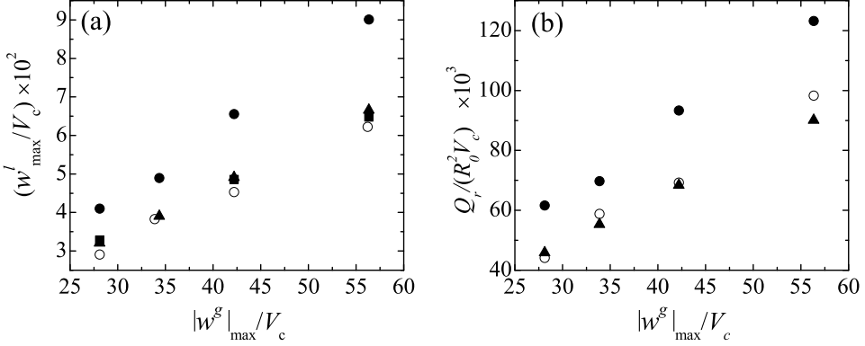
Figure 19: Maximum value w_{max}^l of the axial velocity component measured in the liquid (a) and recirculating flow rate Q_r (b) as a function of |w_{max}^g|_{max} for Bo = 0 (open symbols), Bo = 4.06 (circles), and Bo = -4.06 (triangles). The squares in (a) correspond to the simulations for Bo = 0 with a rigid free surface.
