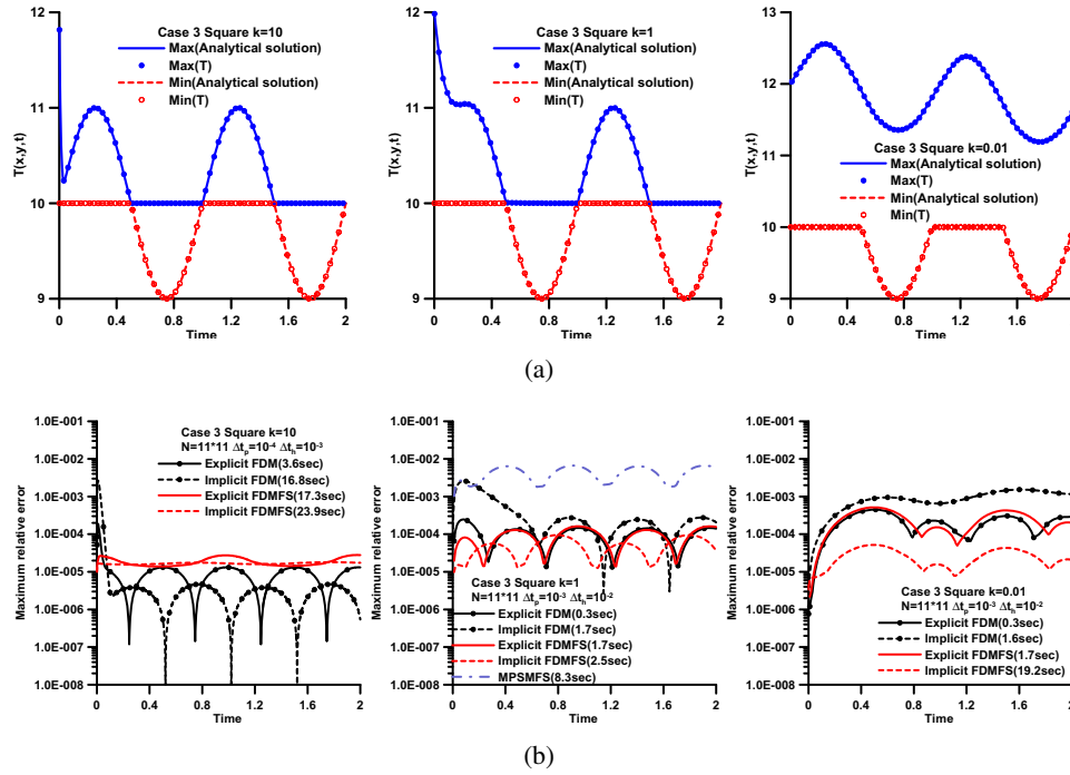
Figure 10: Time history of maximum and minimum temperatures for case 3 when k=10 , k=1 and k=0.01
