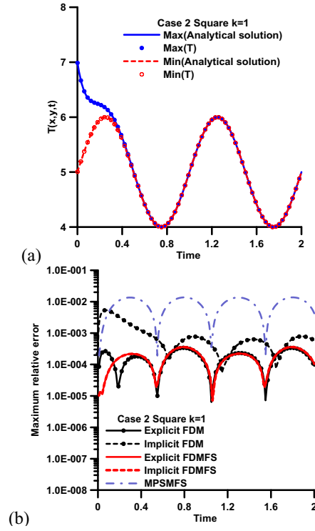
Figure 6: Time history of (a) maximum and minimum values of T and (b) maximum relative error for case 2
