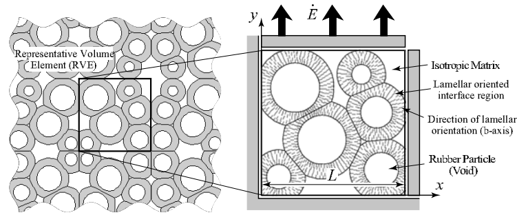
(a) RVE Model of mesostructure of rubber blended semi-crystalline polymer.
