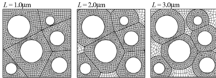
(b) Mesh divisions for each model size.
