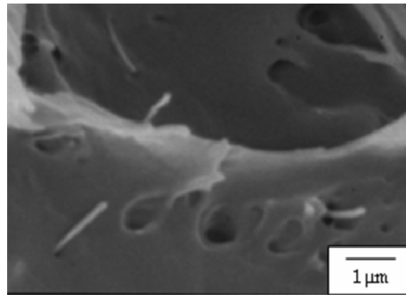
Figure 6: Fracture surface of amorphous composite specimen (10wt%)
