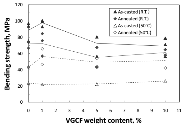
Figure 3: Bending strength
