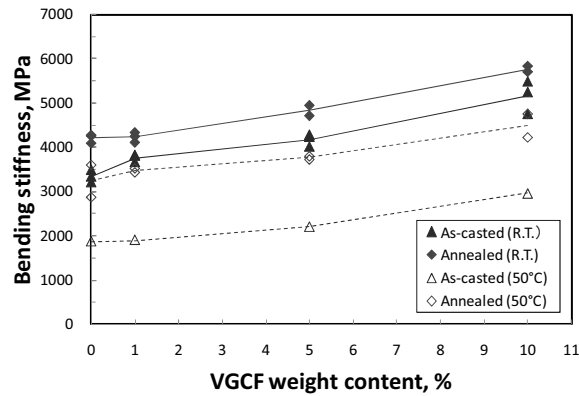
Figure 2: Bending stiffness
