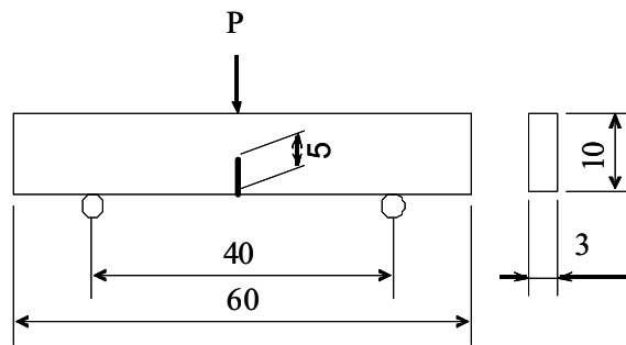
Figure 4: Fracture toughness specimen
