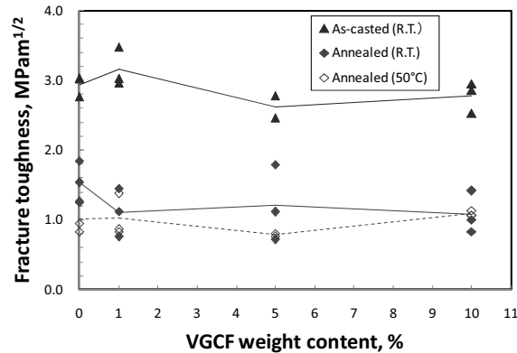
Figure 5: Fracture toughness
