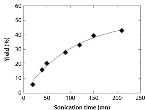
Figure 1 Evolution of the yield of the dispersion process versus the sonication time (initial parameters: ultrasound power 0.7 W/mL, [CNC] = 4 g/L, [SWNT] = 0.5 g/L). The continuous line fits the data with a unimolecular rate law described in the text.
