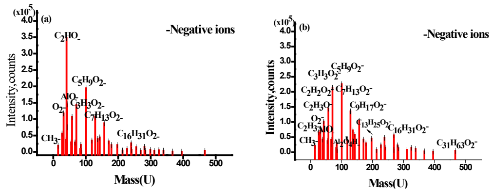
Figure 7: TOF-SIMS spectra of negative ions in the worn surfaces lubricated by (a) neat SE base oil and (b) SE with wheat leaf-surface wax at room temperature
