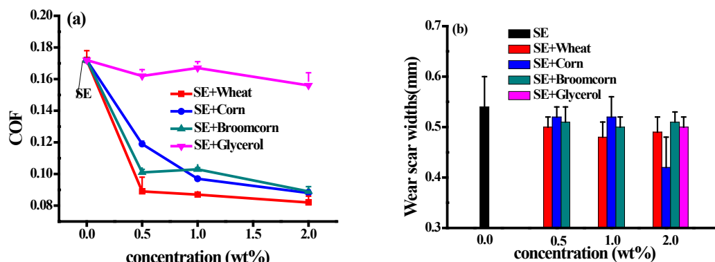
Figure 1: average COFs (a) and wear scar widths (b) for the lubricants for steel-aluminum pair at different additive concentration at 20 N, 5 Hz and RT
