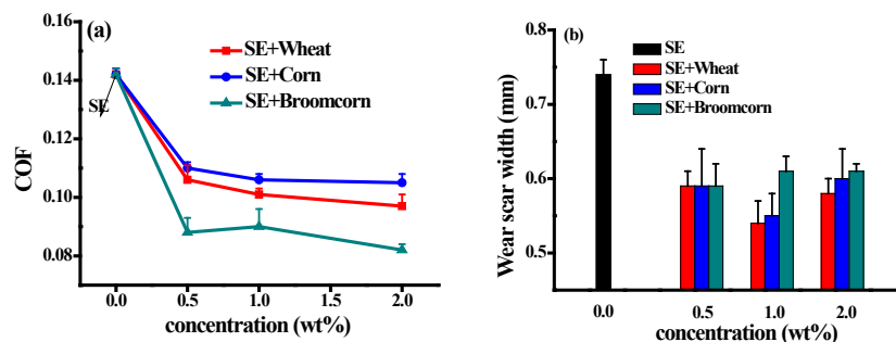
Figure 3: average COFs (a) and wear scar widths (b) for the lubricants for steel-copper pair at different additive concentration at 40 N, 5 Hz and RT
