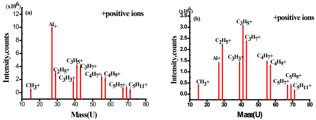
Figure 6: TOF-SIMS spectra of positive ions in the worn surfaces lubricated by (a) neat SE base oil and (b) SE with wheat leaf-surface wax at room temperature
