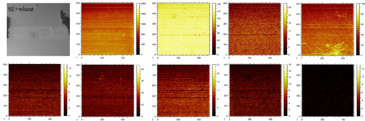
Figure 8: SIMS images of positive and negative ions from a selected area lubricated by the neat SE and SE with wheat leaf-surface wax at room temperature
