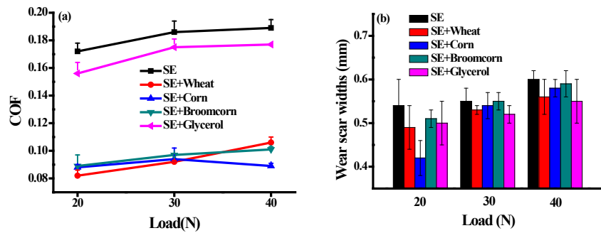
Figure 2: average COFs (a) and wear scar widths (b) for the lubricants for steel-aluminum pair at different loads at 5 Hz and RT
