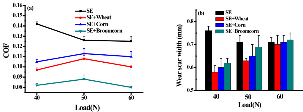
Figure 4: average COFs (a) and wear scar widths (b) for the lubricants for steel-copper pair at different loads at 5 Hz and RT
