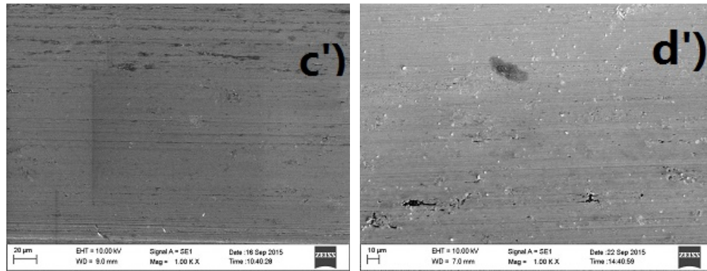
Figure 5: SEM images of the worn surfaces lubricated by (a') SE base oil, (b') broomcorn, (c') corn, and (d') wheat
