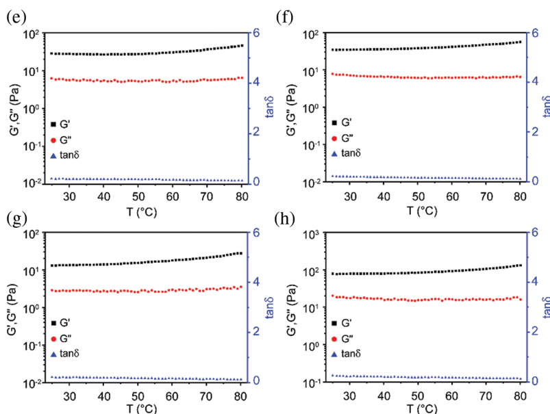
Figure 7: Rheological properties of 0.2 wt% (a, c, e, g) and 0.5 wt% (b, d, f, h) NFC suspensions with increasing the temperature. (a, b) wood, (c, d) sugarcane bagasse, (e, f) rice straw, and (g, h) bamboo
