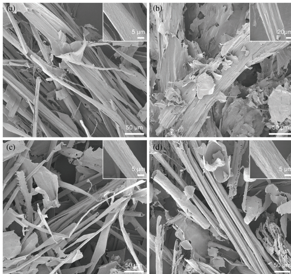
Figure 1: SEM images of the cellulose pulps of (a) wood, (b) sugarcane bagasse, (c) rice straw and (d) bamboo
