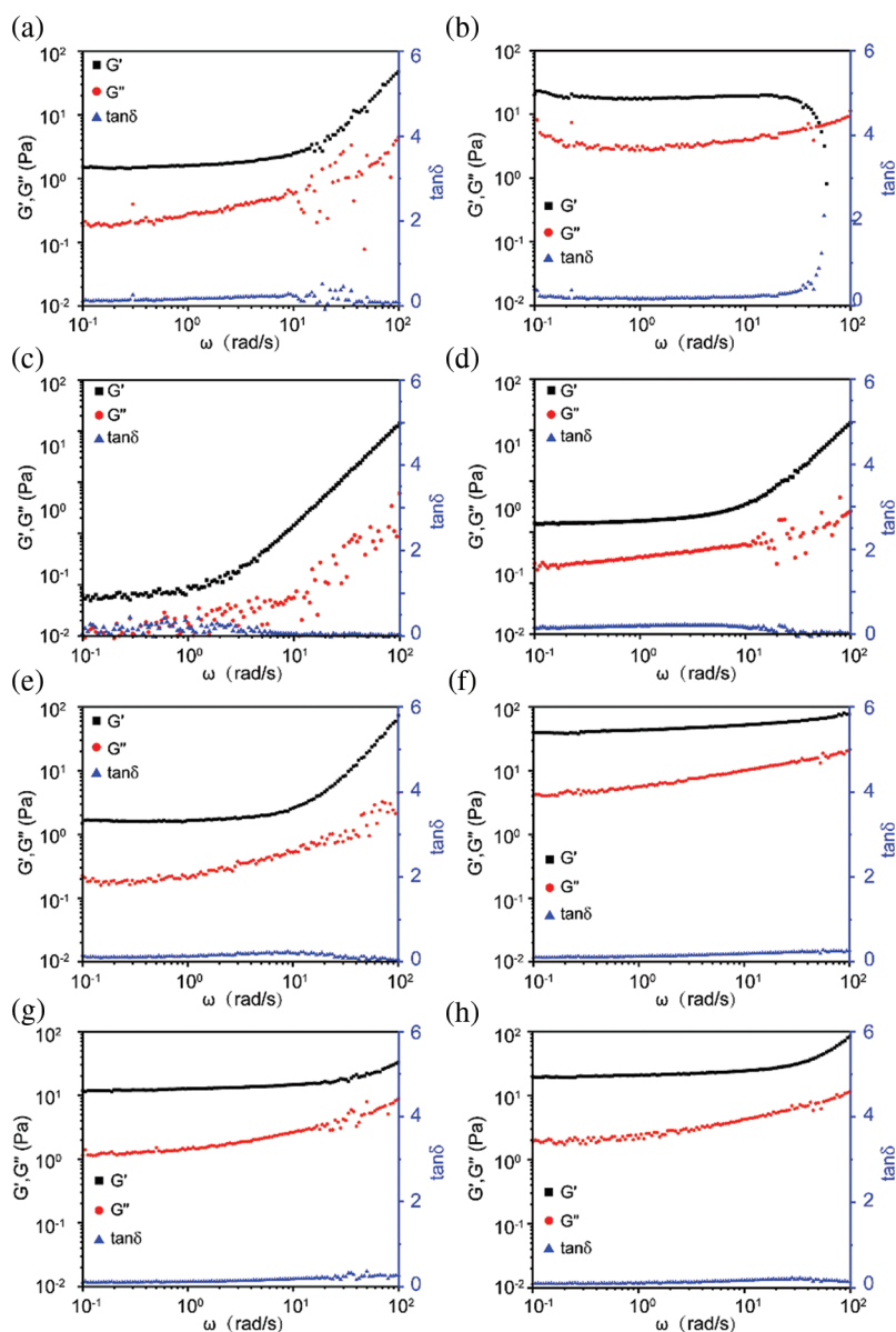
Figure 6: Rheological properties of 0.2 wt% (a, c, e, g) and 0.5 wt% (b, d, f, h) NFC suspensions with increasing the angular frequency. (a, b) wood, (c, d) sugarcane bagasse, (e, f) rice straw, and (g, h) bamboo
