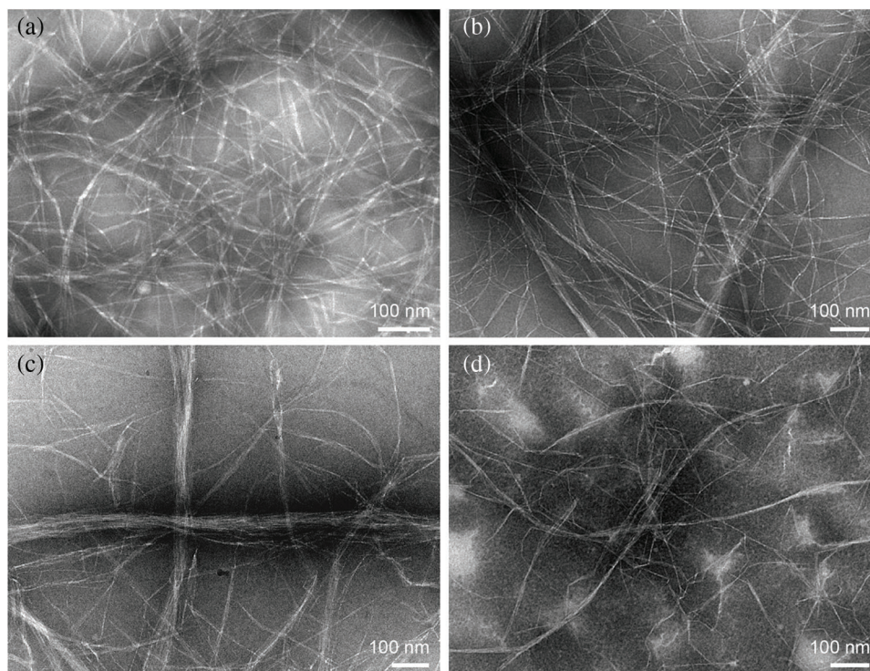
Figure 2: TEM images of NFC isolated from the PCPs of (a) wood, (b) sugarcane bagasse, (c) rice straw and (d) bamboo
