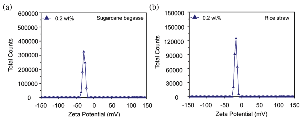
Figure S2: Determination of Zeta potential on NFCs. (a) Sugarcane bagasse, (b) rice straw
