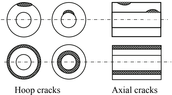
Figure 2: All crack configurations considered in the analyses
