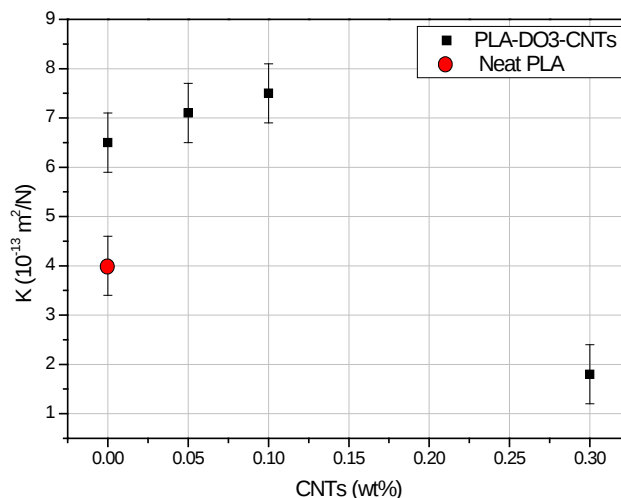
Figure 4: Wear coefficient for all developed materials
