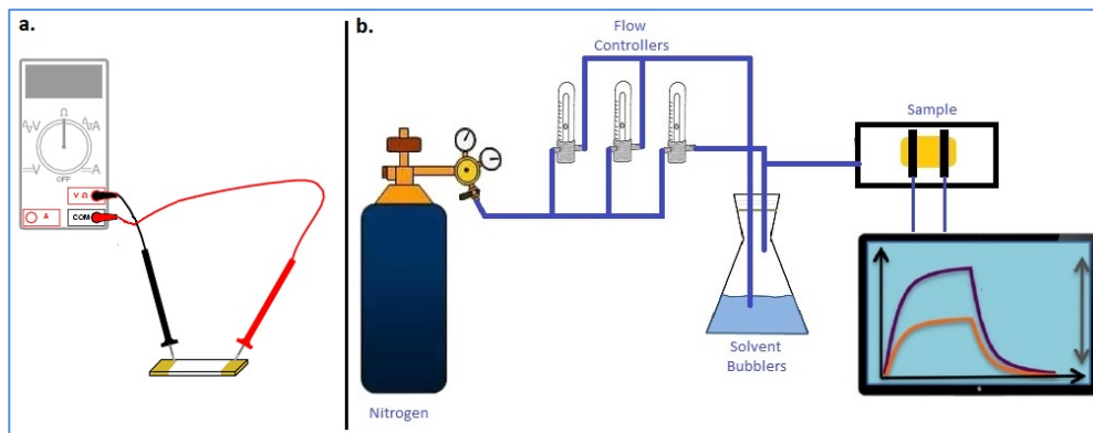
Figure 1: a. Scheme of electrical resistance measurement. b. Scheme of vapor sensing device
