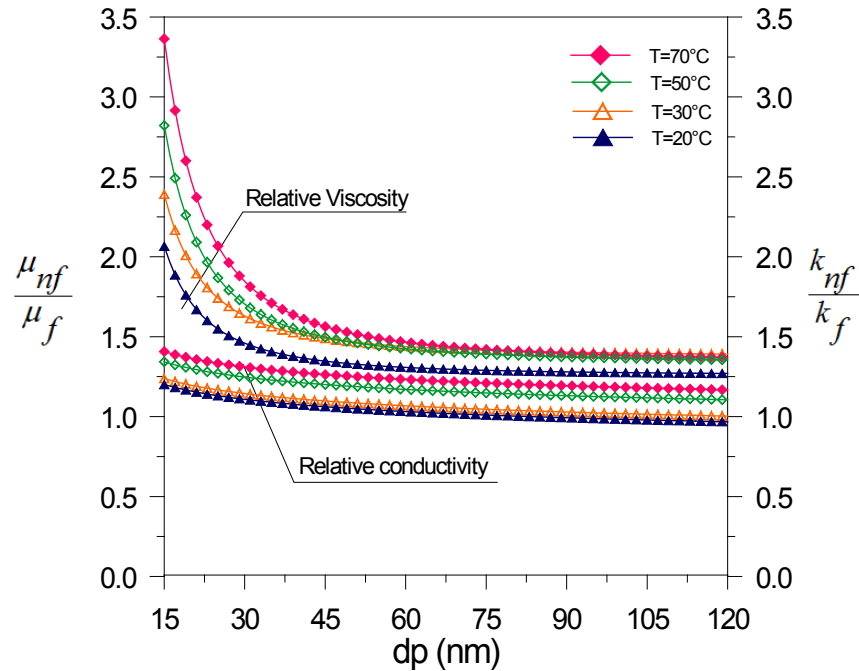
Figure 10: Effect of diameter size in relative viscosity and relative thermal conductivity of \text{Al}_2\text{O}_3 -water nanofluid for different temperatures
