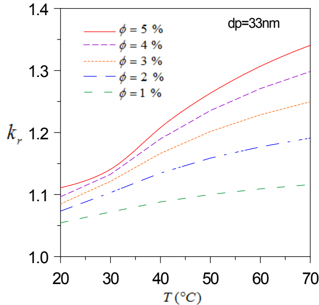
Figure 6: Variation of the relative thermal conductivity Al 2 O 3 -water versus temperature
