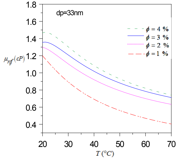
Figure 7: Variation of the viscosity versus temperature
