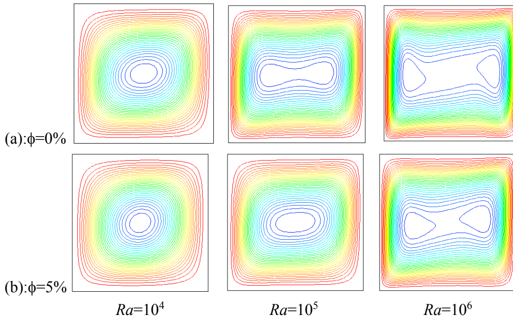
Figure 5: Streamlines for the cavity filled with Al_2O_3 -water nanofluid at Ra=10^4 , 10^5 and 10^6 ; (a): \phi=0\% , (b): \phi=5\%
