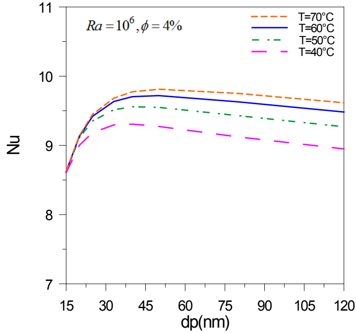
Figure 11: Influence of nanoparticle's diameter of Al_2O_3 on Nusselt number
