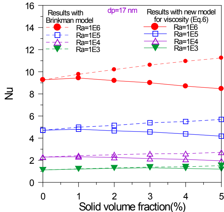
Figure 4: Effect of the solid volume fraction of Al_2O_3 -water nanofluid with different Rayleigh numbers on the Nusselt number via a comparison between our models (continuous curves) and Brinkman model for viscosity (discontinuous curves)
