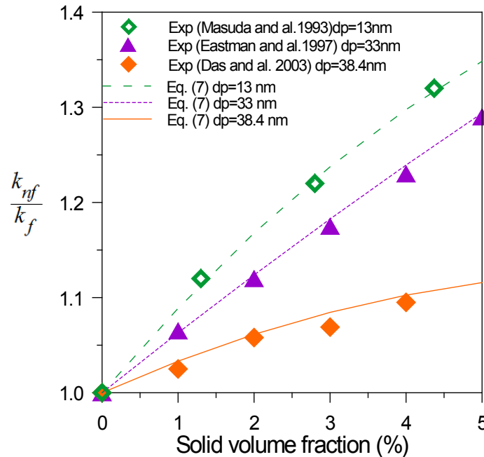
Figure 2: Comparison of the proposed model with those experiments for Al 2 O 3 -water thermal conductivity
