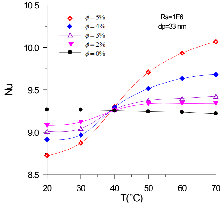
Figure 8: Effect of temperature on Nusselt number for different volume fractions of Al_2O_3
