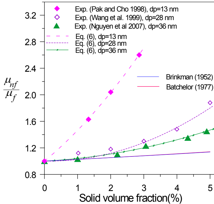
Figure 1: Comparison of the new model of viscosity \text{Al}_2\text{O}_3 -water model to experiments data: Curves corresponding to theoretical models [Batchelor (1977); Brinkman (1952)] are confounded for this scale of \mu_{nf}/\mu_f
