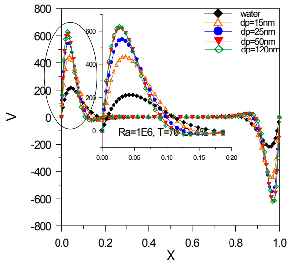
Figure 12: Velocity profile at midplane cavity at Ra=10^6 and T=70^\circ C , for various nanoparticles sizes
