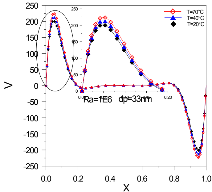
Figure 9: Velocity profile at midplane cavity ( y=0.5 )
