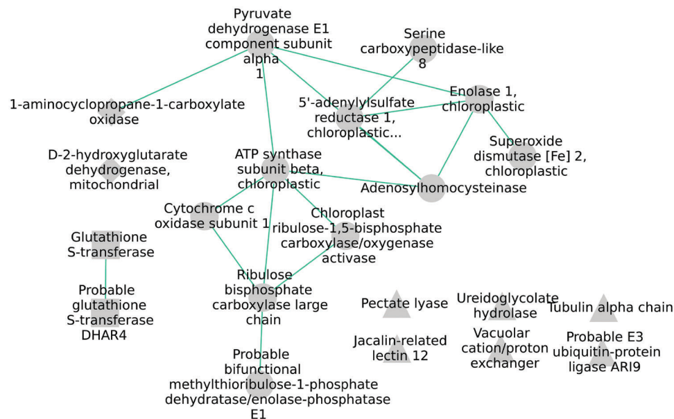
Figure 2: The PPI network of identified DAPs in canola leaves under severe drought stress. The network includes all DAPs and interactions between them. PPI and extended PPI of DAPs constructed using STRING 11.0 with confidence score of >0.70
