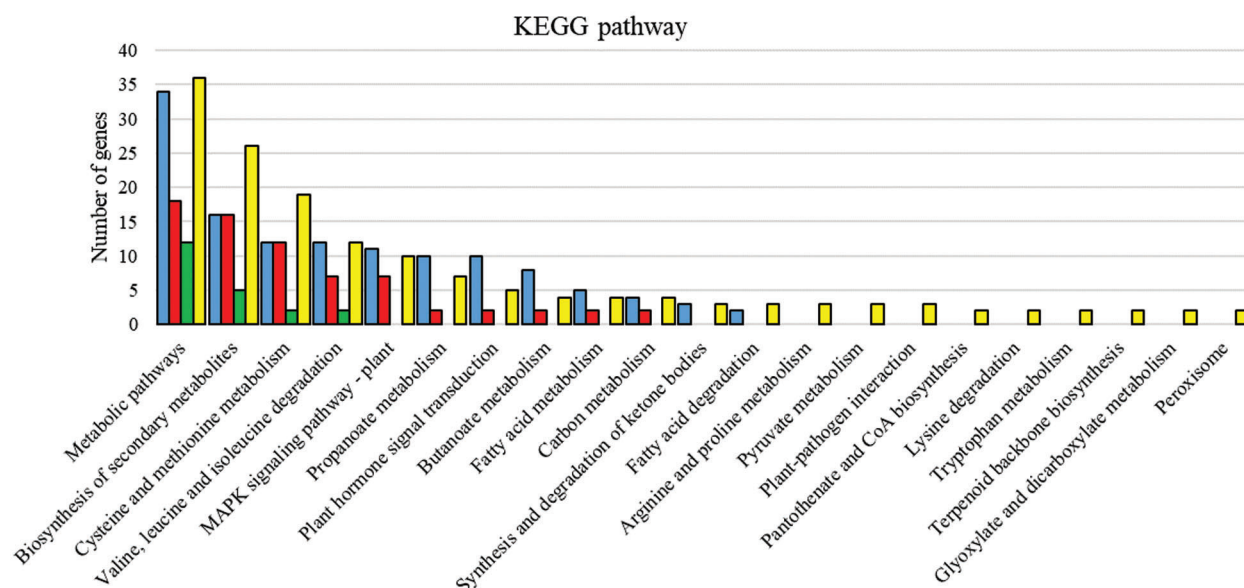
Figure 7: KEGG analysis of the extended networks. The blue, red, green, and yellow bars indicate the first, second, third, and fourth groups, respectively
