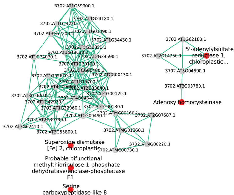
Figure 3: The 4th extended network of the first group of DAPs and their interactions with neighbors. PPI and extended PPI of DAPs constructed using STRING 11.0 with confidence score of >0.70
