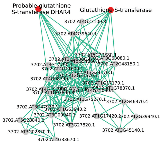
Figure 4: The 4th extended network of the second group of DAPs and their interactions with neighbors. PPI and extended PPI of DAPs constructed using STRING 11.0 with confidence score of >0.70
