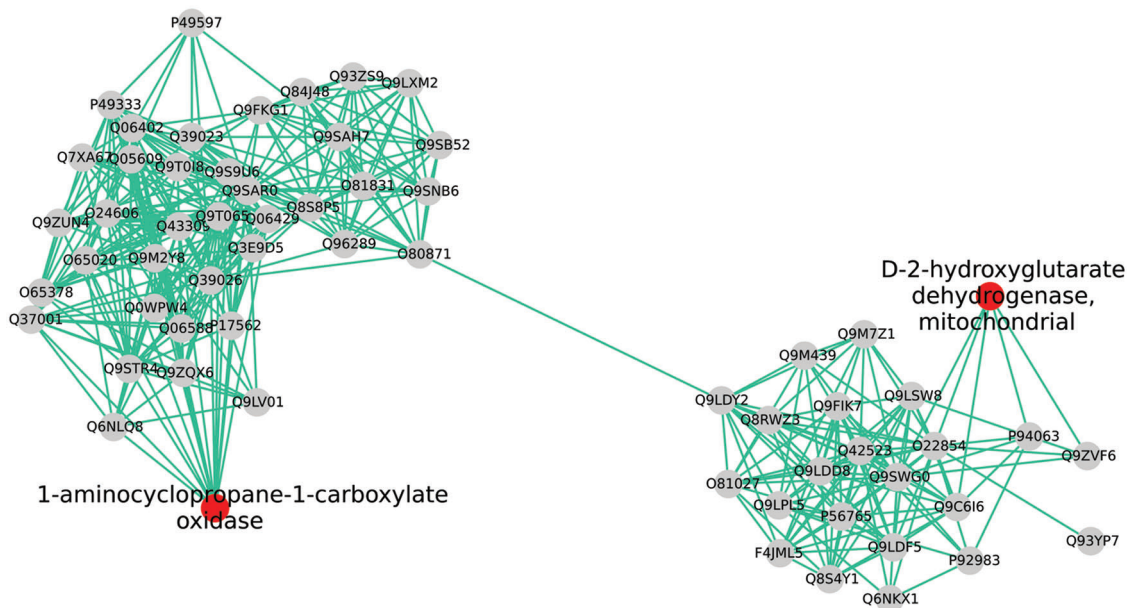
Figure 6: The 6 th extended PPI network of 1-aminocyclopropane-1-carboxylate oxidase (Q09052) and D-2-hydroxyglutarate dehydrogenase, mitochondrial (O23240). This network includes two DAPs with increased abundance under drought stress and their neighbors from STRING database. The extended network was constructed using STRING 11.0 with a confidence score of >0.70
