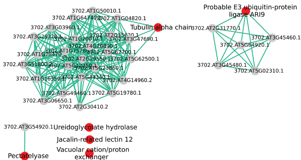
Figure 5: The 4th extended network of the third group of DAPs and their interactions with neighbors. PPI and extended PPI of DAPs constructed using STRING 11.0 with confidence score of >0.70
