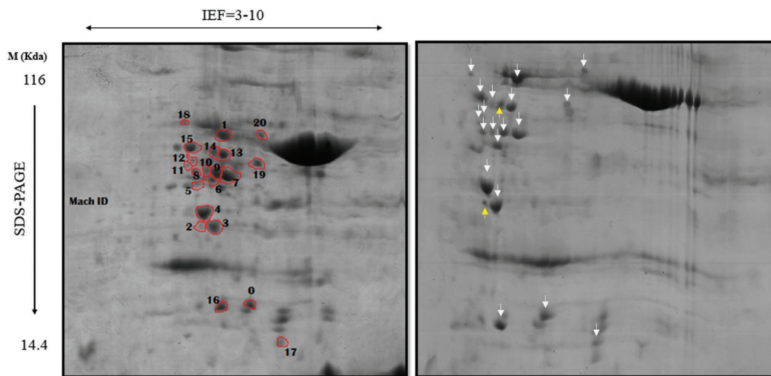
Figure 1: Differentially abundant proteins (DAPs) in the leaves of canola under control (left) and treated samples with severe drought stress (right). Spot numbers refer to IDs of identified proteins detailed in Table 1. Total protein of canola leaves (350 \mu l) was separated in two dimensions. First according to the isoelectric point and then according to the size of proteins. Up and down arrows show increased and decreased abundance
