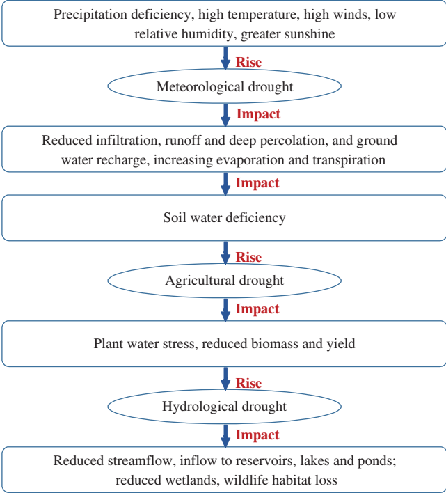
Figure 1: Origin and flow of drought
