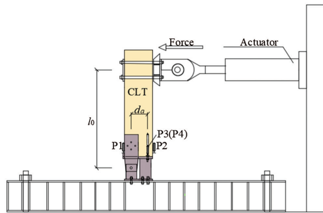
Figure 4: Loading and measuring device
