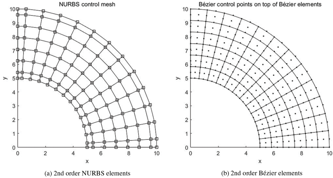
Figure 3: Circular beam, meshes of IGA, NURBS and Bézier physical mesh with control points
