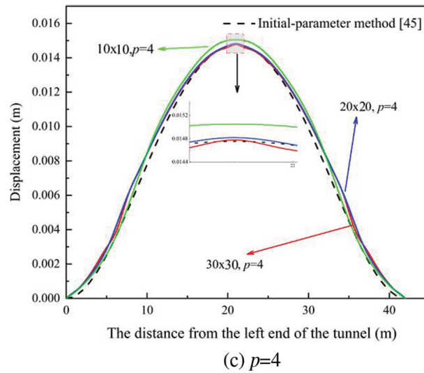
Figure 12: Interval tunnel loaded by a uniform pressure: displacement of each point and convergence to the initial parameter solution in the third situation
