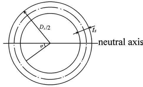
Figure 8: Schematic diagram of neutral axis position
