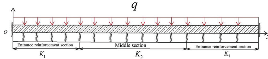
Figure 9: Interval tunnel calculation model
