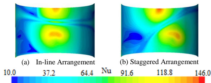
Fig. 13 Nu number distributions on the moving curved surface at Re=23000 , H/d=5 , S/d=4 , Cr=0.8 and VR=0.28
