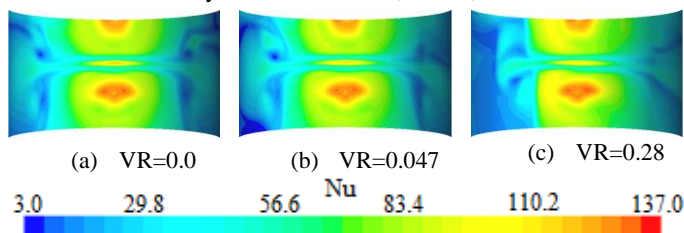
Fig. 18 Nusselt number distributions on the moving curved surface for different velocity ratio at Re=23000 , H/d=2 , S/d=4 and Cr=0.8
