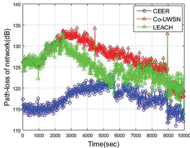
Figure 6: The Path Loss vs. Time (Sec)
