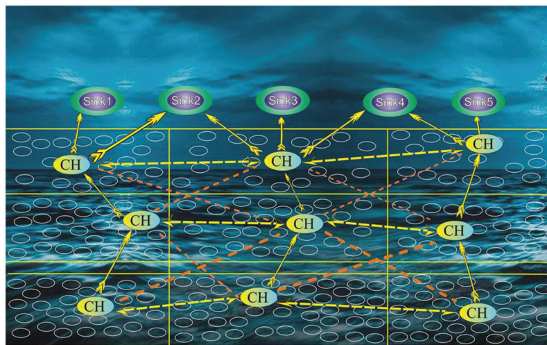
Figure 2: Cooperative Energy Efficient Routing (CEER) Cluster-based Protocol
