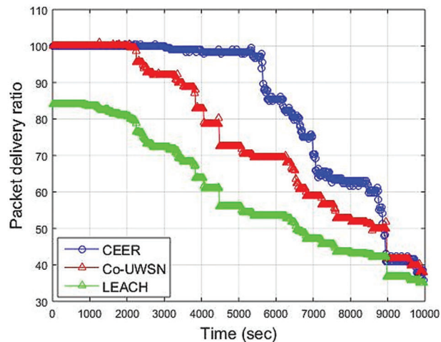
Figure 5: Packet Delivery Ratio vs. Time (Sec)
