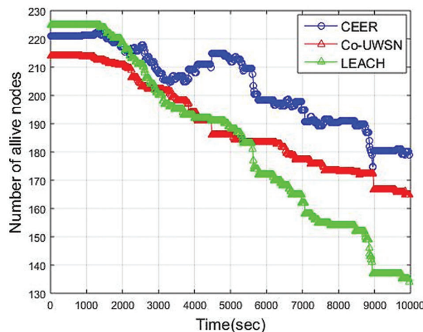
Figure 7: Alive nodes vs. network Lifetime (Sec)
