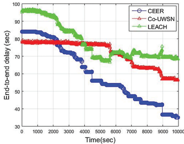
Figure 3: End-to-End Delay vs. Time (Sec)
