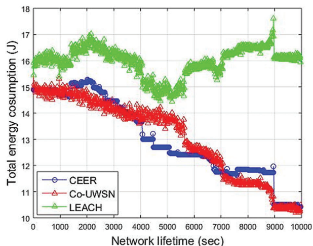
Figure 4: Total Energy Consumption vs. Time (Sec)
