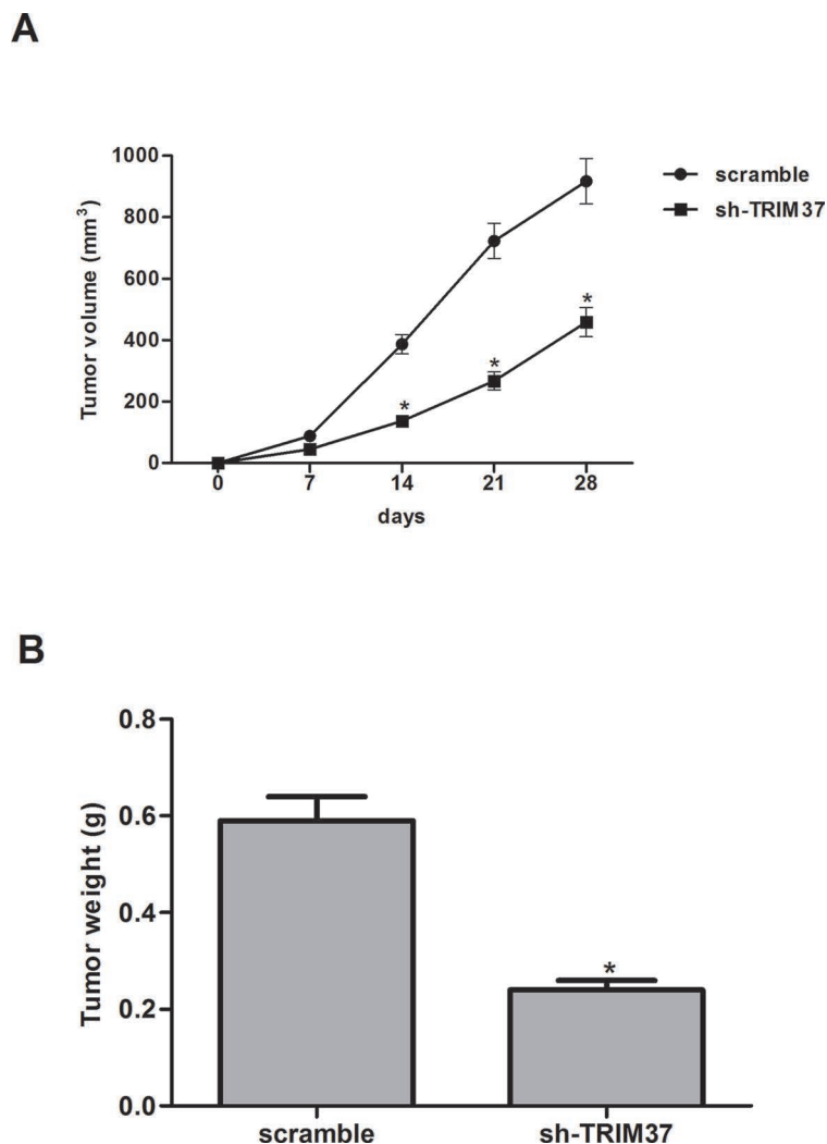
Figure 3. Knockdown of TRIM37 inhibits tumor growth in vivo. Infected HCT116 cells ( 1 \times 10^6 ) were injected subcutaneously into the right hindlimb of 4-week-old nude mice. (A) The tumor volume was monitored every week and measured. (B) After 4 weeks, the mice were sacrificed, and the tumors were dissected out and weighed. Data are mean \pm SD from three independent experiments. * p < 0.05 versus scramble group.
