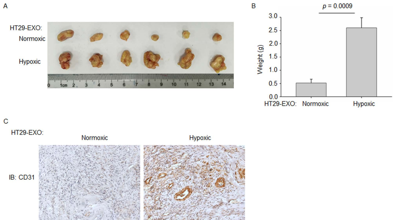
Figure 6. The role of CRC derived-exosomal Wnt4 promoted tumor growth and angiogenesis. (A) Photo of tumors inoculated with HT29 cells subcutaneously with exosome treatment. (B) Tumor weight of formed tumors inoculated with HT29 cells subcutaneously with exosome treatment. (C) Immunohistochemistry analysis of CD31 showed that angiogenesis was higher in hypoxic exosome-treated tumor. Magnification: 200 \times .
