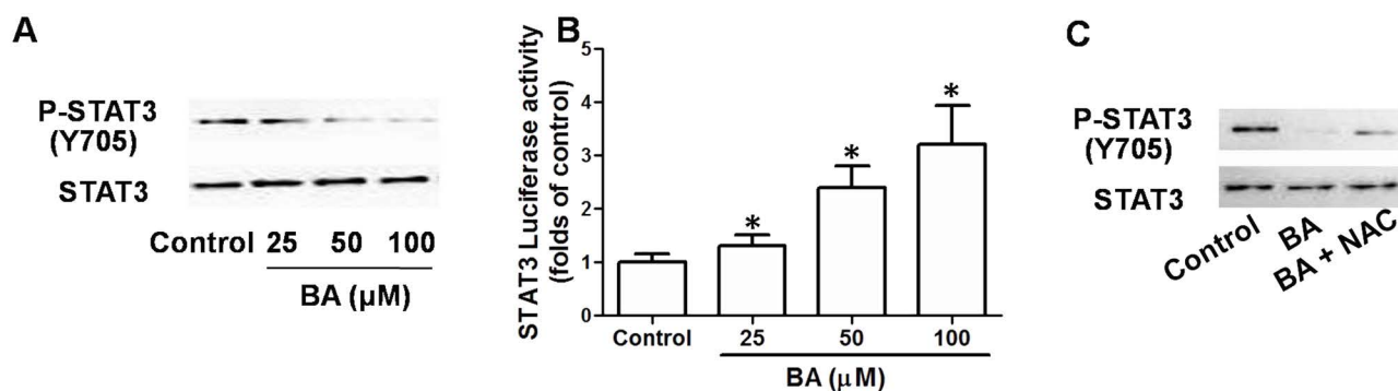
Figure 6. Role of inhibition of signal transducer and activator of transcription 3 (STAT3) signaling in the antitumor effect of BA in vitro. KB cells were incubated with indicated concentrations of BA for 24 h. (A) Phosphorylation of STAT3 was determined by Western blot. (B) Reporter gene activity of STAT3 was examined and shown as a relative activity of the control group. KB cells were exposed to 100 μM BA in the presence or absence of 100 μM NAC for 24 h. Phosphorylation of STAT3 was determined by Western blot (C). * p < 0.05 , compared with that of the control.
